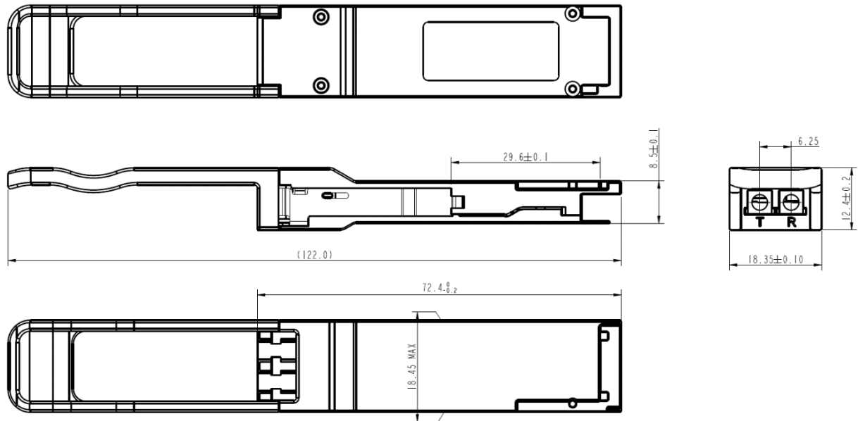
Figure 3. Mechanical Dimensions
